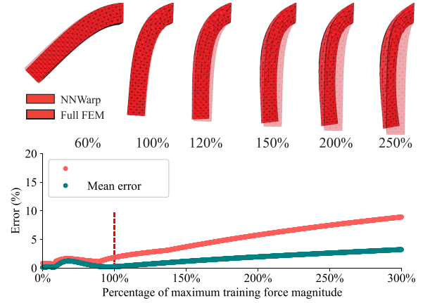
Fig. 18. Extrapolation errors when the force magnitude exceeds the training coverage.
