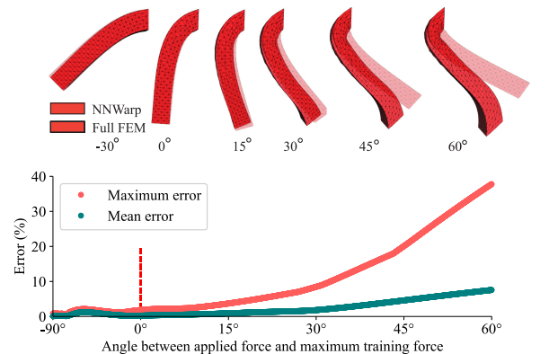
Fig. 19. Extrapolation errors when the force direction exceeds the training coverage.
