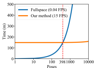
Fig. 14. The training effort is paid off for an animation of moderate length.
