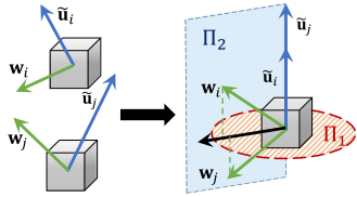
Fig. 12. Rotation invariance allows us to further compress the input kinematic feature.
