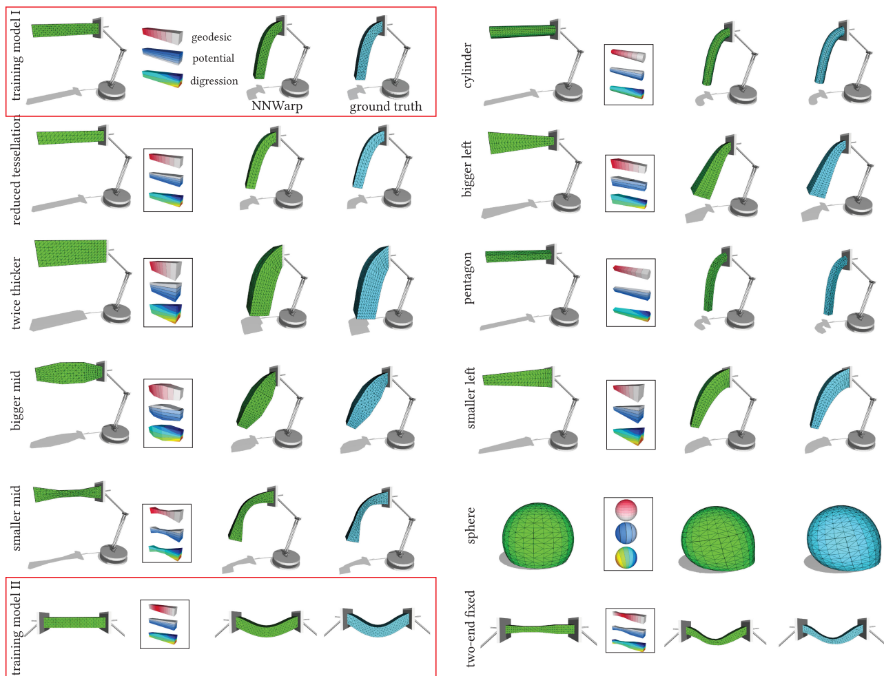
Fig. 6. We test the generality of the designed features on a variety of shapes. The training data are generated using the standard rectangular beam (highlighted by a red box). The resulting DNN successfully handles many beam-like models but with distinctively different shapes. The distributions of three features are also plotted.
