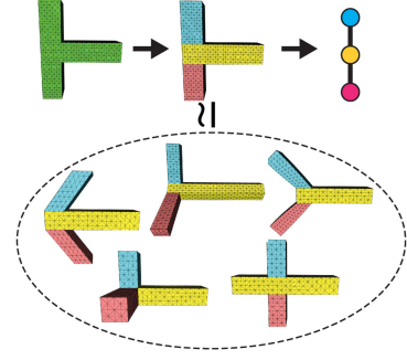
Fig. 10. Building domain graph for the domain decomposed model is an easy and effective way to identify shapes with similar concavity.
