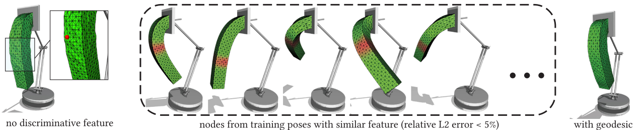
Fig. 4. Only using kinematic feature as the input of the network yields noticeable jittery artifacts. A node, because of its kinematic feature is not discriminative, could be influenced by many irrelevant instances in the training data. Large discrepancies among these mismatched nodes induce high-frequency variations of the NNWarp. Incorporating geodesic feature effectively eliminates this artifact.
