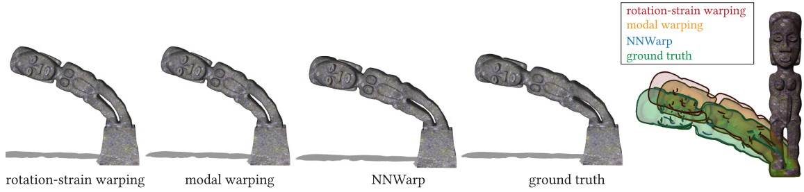
Fig. 13. A side-by-side comparison shows a clear advantage of NNWarp over the existing warping techniques. Its data-driven nature makes the result almost identical to the ground truth while the simulation is as fast as the linear elasticity. The training still uses the rectangular beam model.
