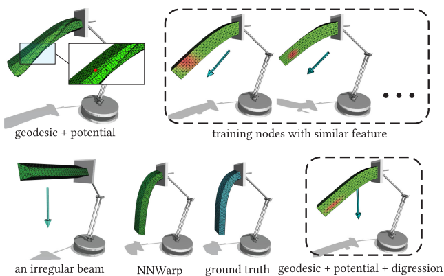
Fig. 7. In order to make NNWarp re-usable for various deformable bodies, we use the digression as our third discriminative feature. With this feature included, the neural network is able to handle an irregular beam based on the training set generated using a standard rectangular beam model.
