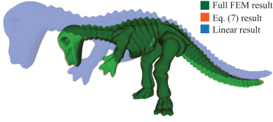
Fig. 3. In practice, Eq. (7) yields good approximations of full nonlinear FEM simulation.
