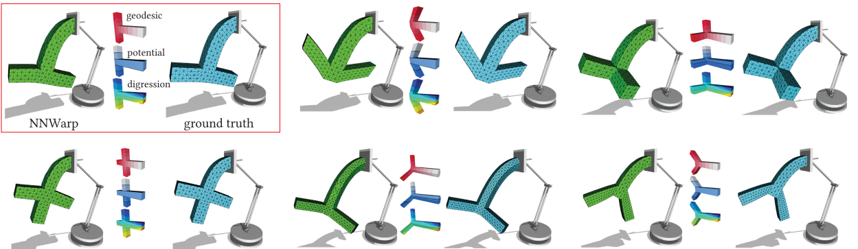
Fig. 11. While a simple rectangular beam is not able to handle highly concave shapes, by referring to the domain graph we can train a network using a T-shape beam and the resulting network can be used to warp a wide range of concave beams whose domain graphs are isomorphic to the T-shape beam.
