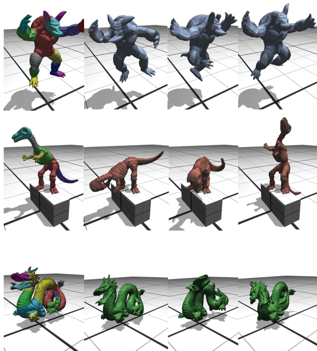
Fig. 16. Substructuring allows us to re-use the training data of a regular shape to handle complex deformable bodies. The Armadillo, dinosaur and dragon models use the StVK, co-rotation and Neo-Hookean materials respectively. They use the networks trained with the rectangular beam.
