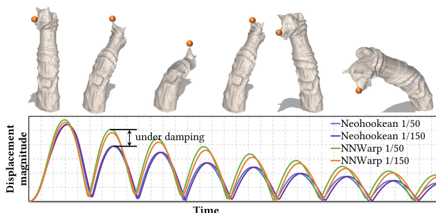
Fig. 15. The deformable motion trajectory (at the nose tip of the wolf head) generated using NNWarp well matches the ground truth under different time step sizes. The vibration frequency resembles the ground truth as well. We use the Newmark integrator in this example.
